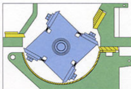
Cutting chamber 粉碎室示意圖
